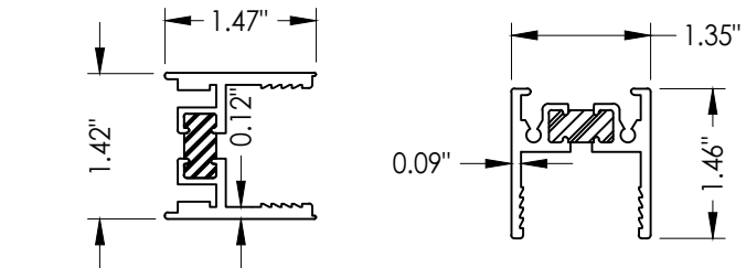
6 TOP RAIL
